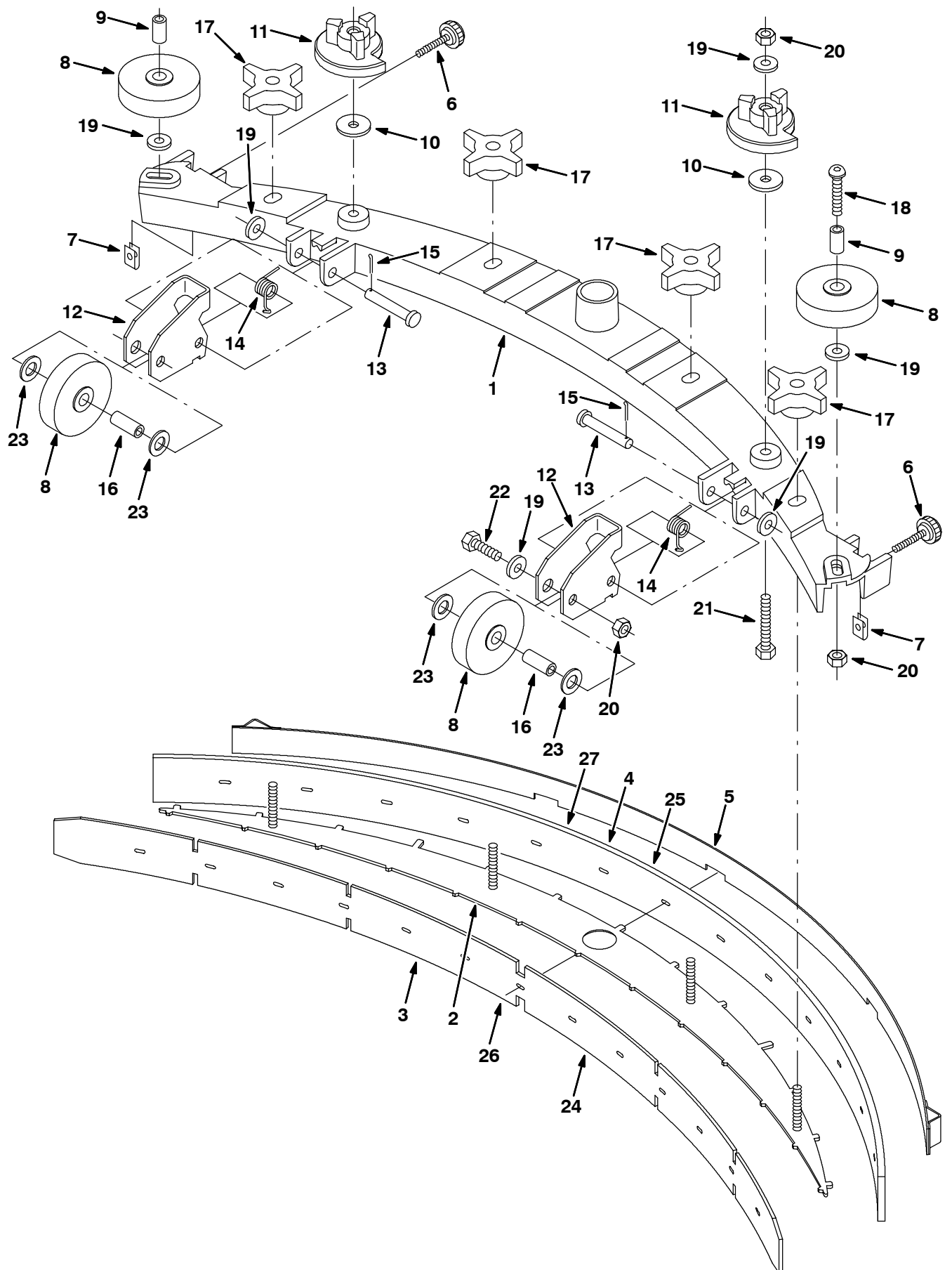
FIG. 2 - Model 900 Squeegee Group, 900 mm (36 in)
